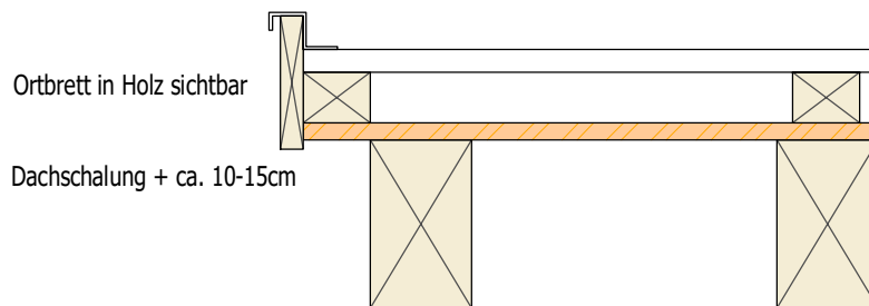
Ortgangdetail Aluverbundplatten
